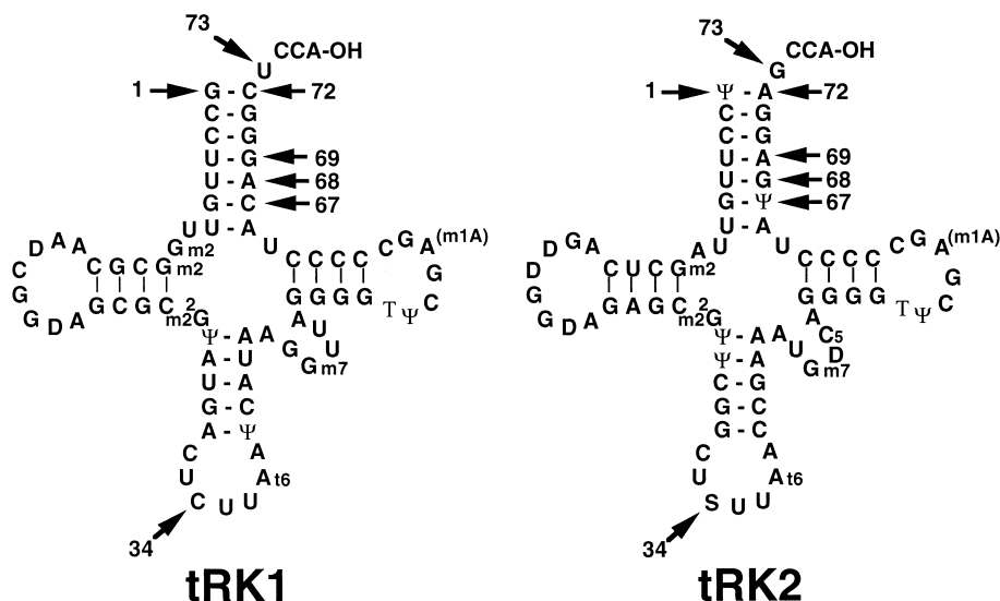
Fig. 1. Cloverleaf structures of tRK1 and tRK2 (based on [8]). Bases that differ between the two isoacceptors in the anticodon loop and aminoacceptor stem are indicated with arrows.
